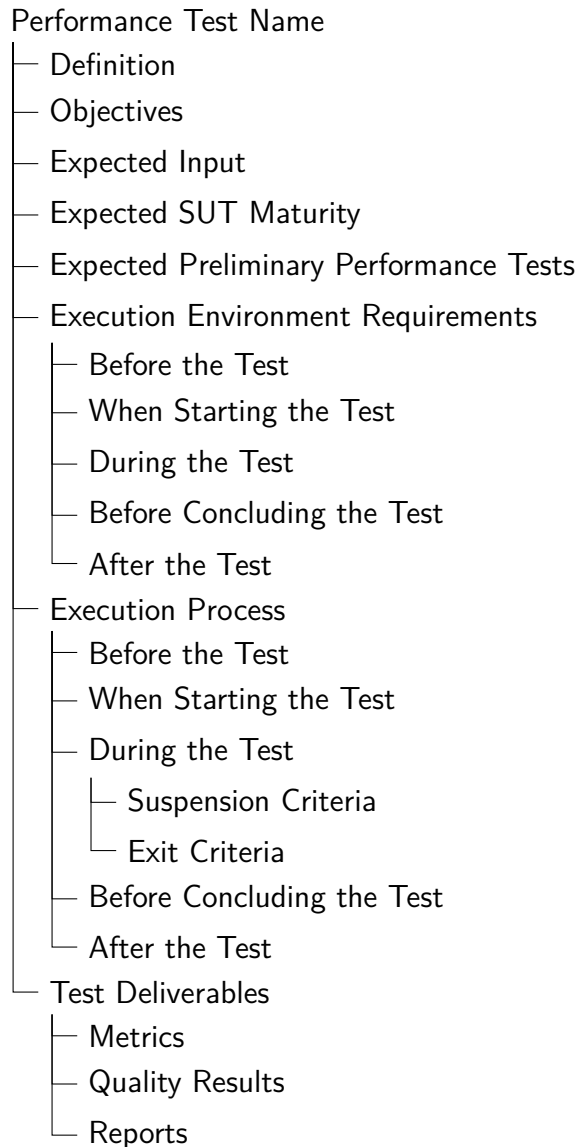
Listing 4.1. The Performance Tests Catalog Template
