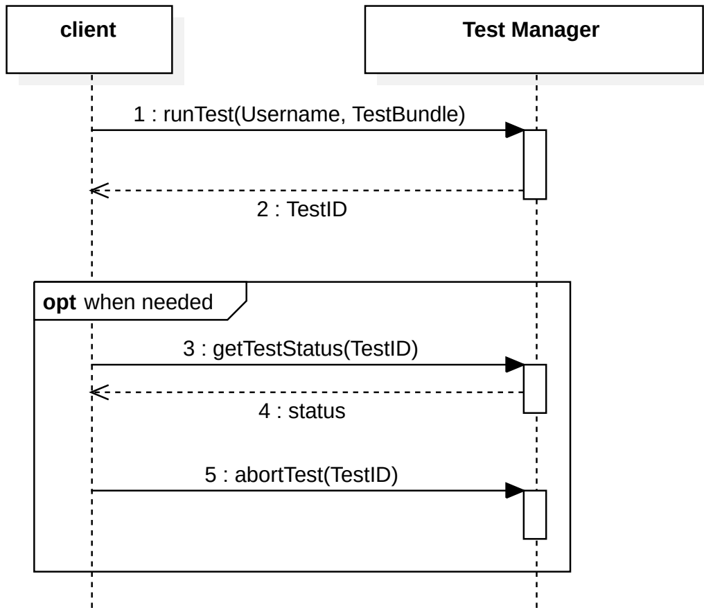
Figure 6.10. BenchFlow Framework: Client Process Sequence Diagram
