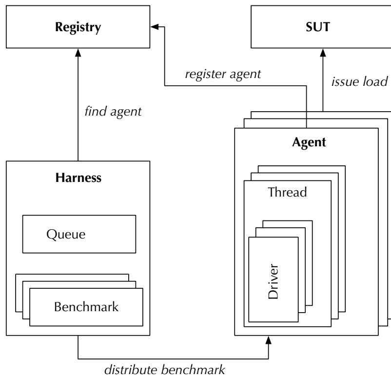
Figure 6.25. Faban Architecture
