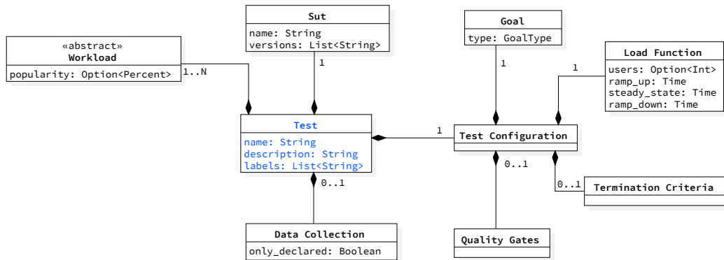
Figure 5.1. DSL: The Test Meta-Model
