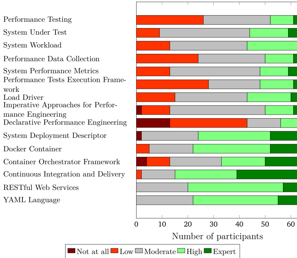
Figure 7.12. Summative Evaluation: Familiarity with Concepts
